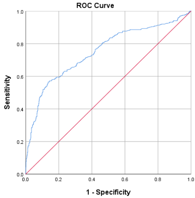
Figure 1: ROC curve: A tool for measuring the multivariate logistic regression model goodness of fit.
